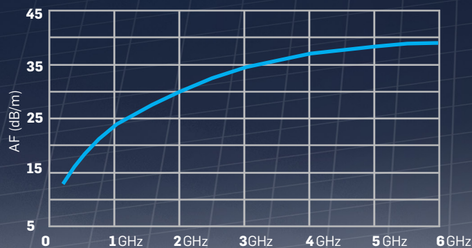
LP-04 - Antenna Factor
