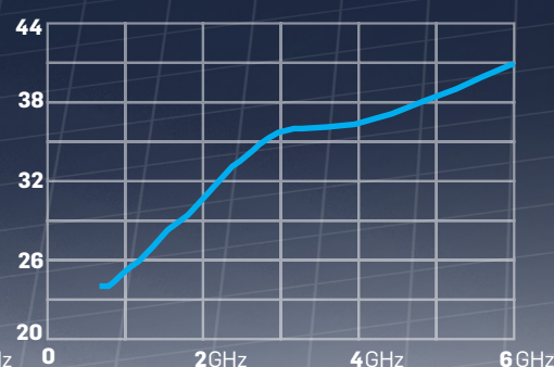
LP-03 - Antenna Factor
