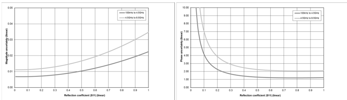
Typical accuracy of reflection magnitude and reflection phase measurements for the R&S® ZND Analysis conditions: S_{12} = S_{21} = 0 , cal. power –10 dBm, meas. power –10 dBm.
