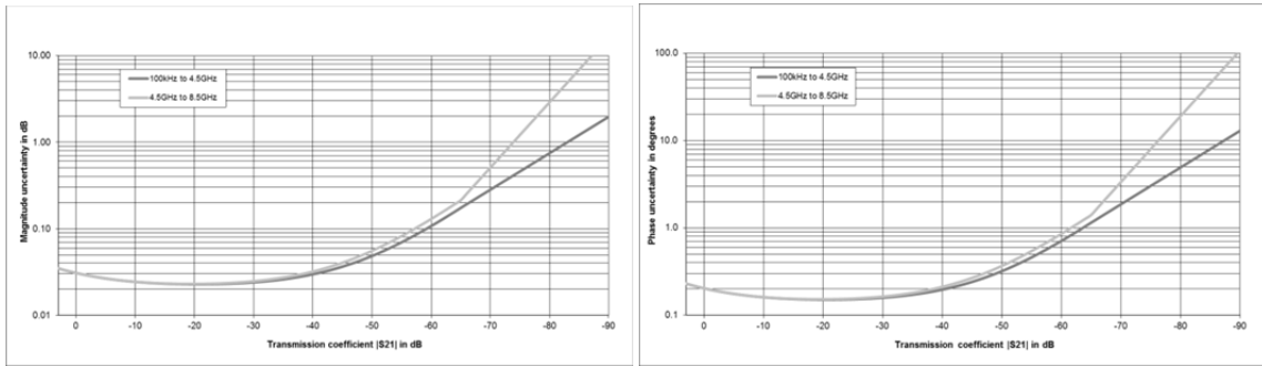
Typical accuracy of transmission magnitude and transmission phase measurements for the R&S® ZND Analysis conditions: S_{11} = S_{22} = 0 , cal. power –10 dBm, meas. power –10 dBm.
